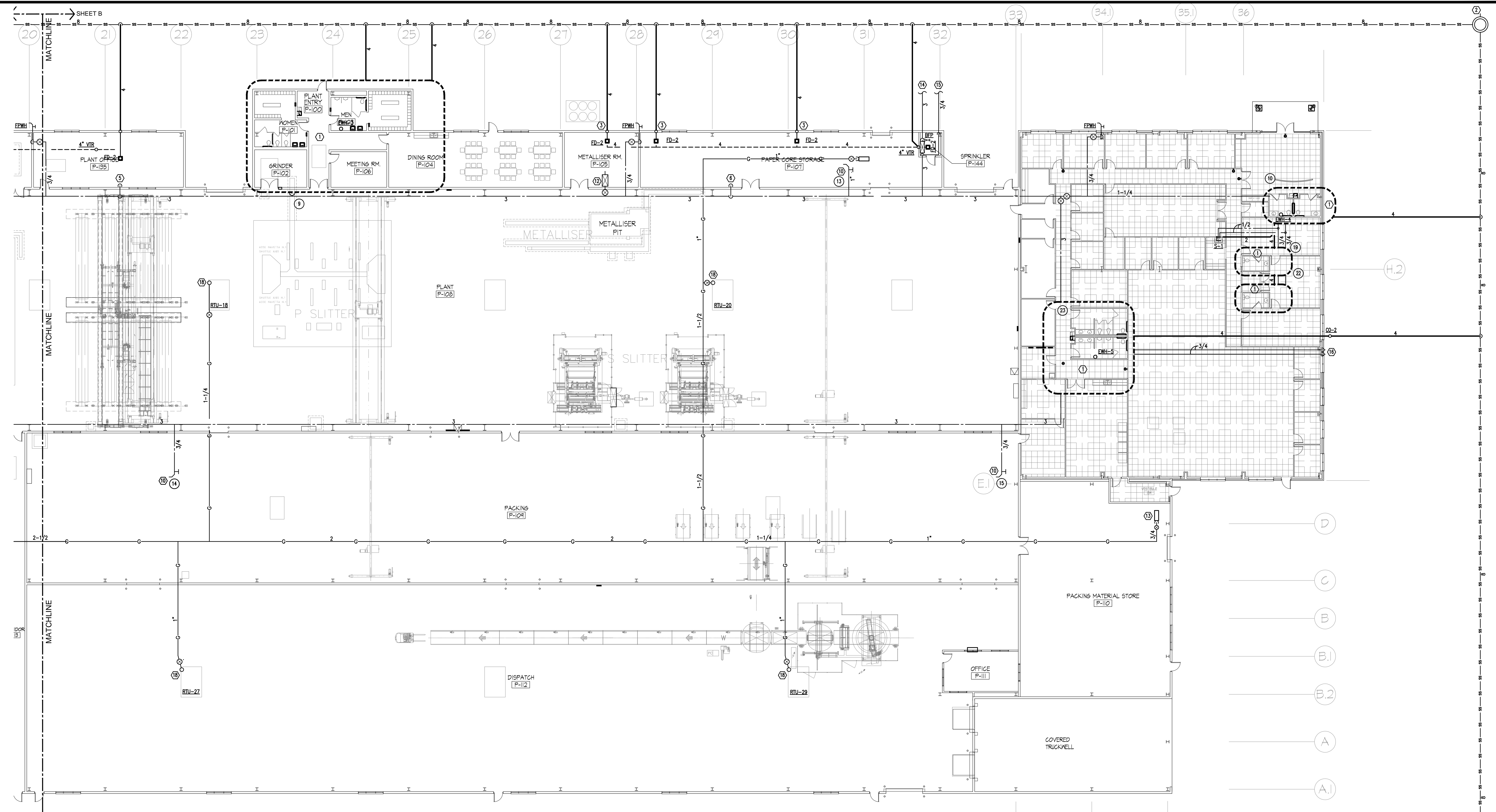
PARTIAL FIRST FLOOR PLUMBING PLAN SCALE: 1/16" = 1'-0"
